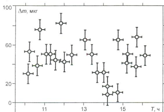
Fig. 2. Mass difference \Delta m (mcg) of the cylindrical titanium rod measured in day-time in its vertical and horizontal orientations.
